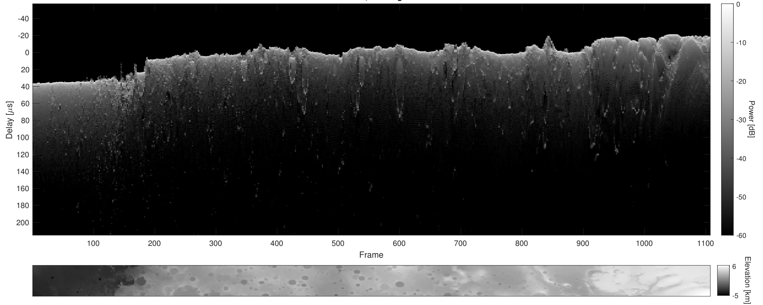
Orbit 6960, Cluttergram
