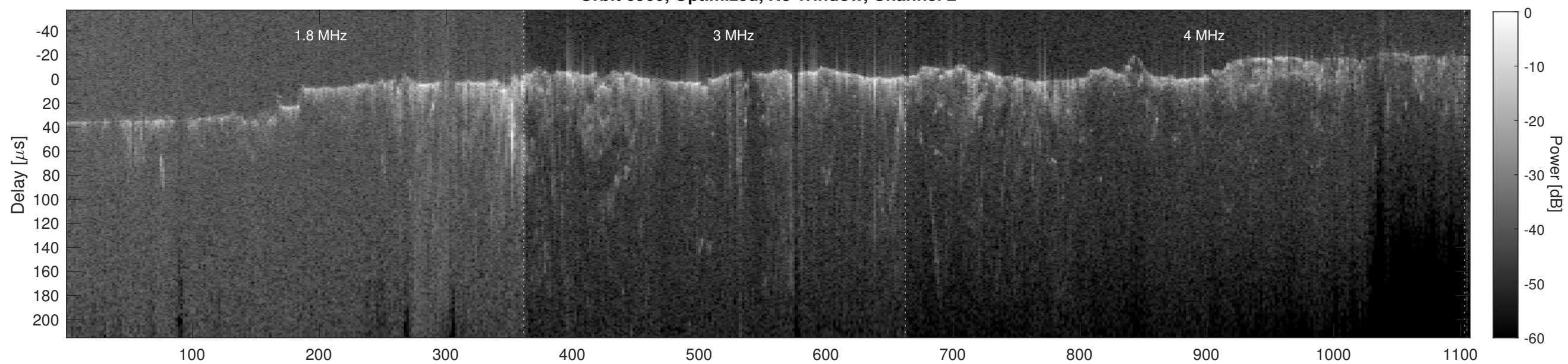
Orbit 6960, Cluttergram
