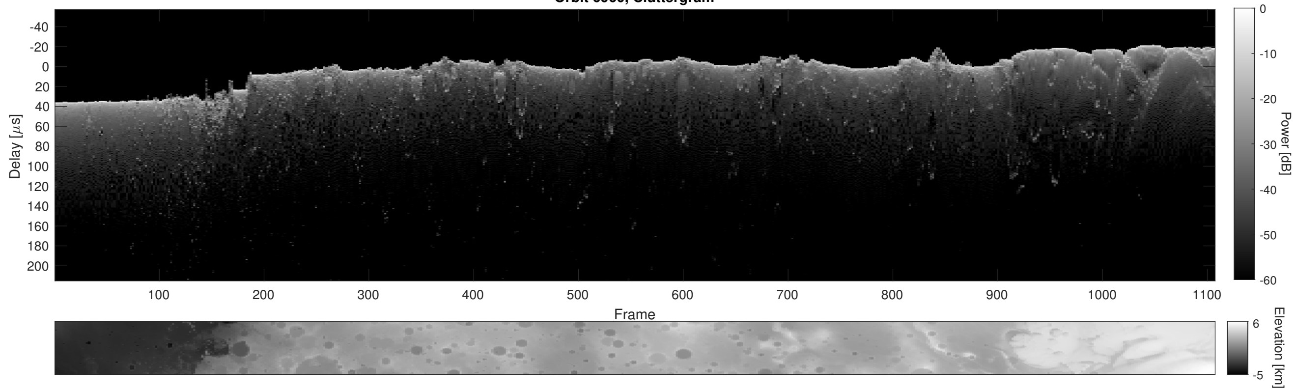
Orbit 6960, Cluttergram
