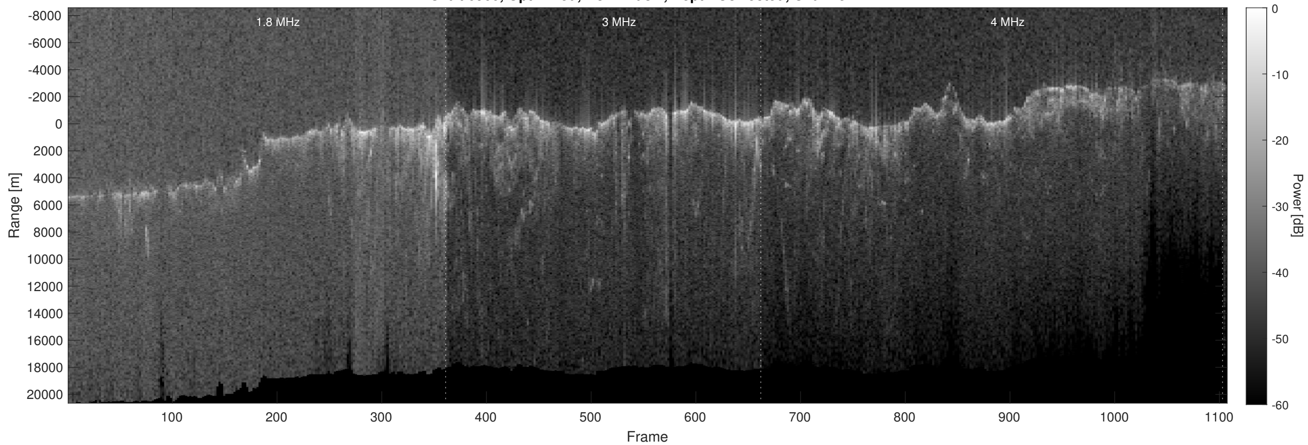
Orbit 6960, Optimized, No Window, Depth-Corrected, Channel 2
