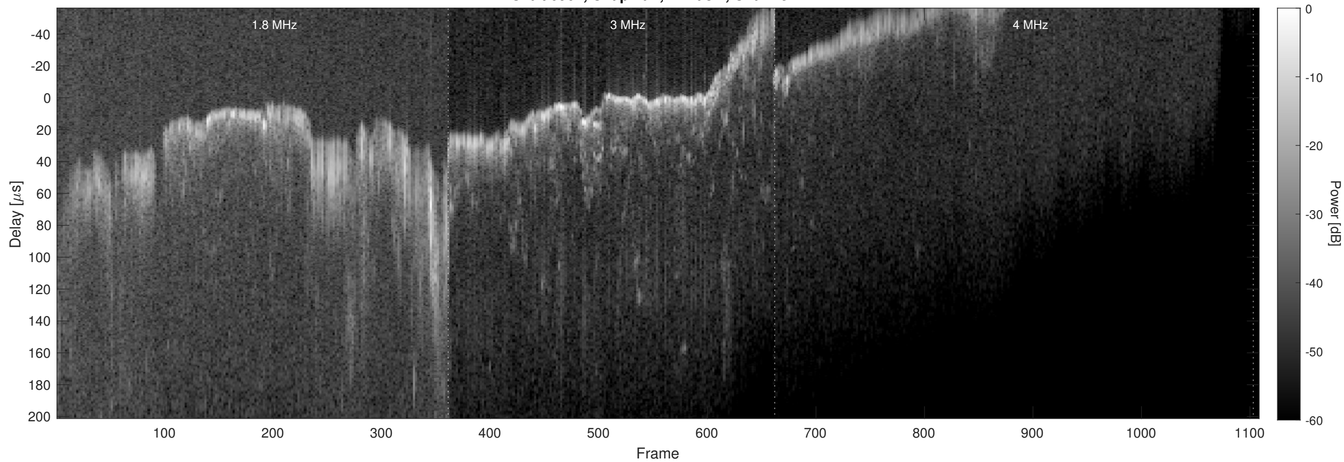
Orbit 6961, Chapman, Window, Channel 2
