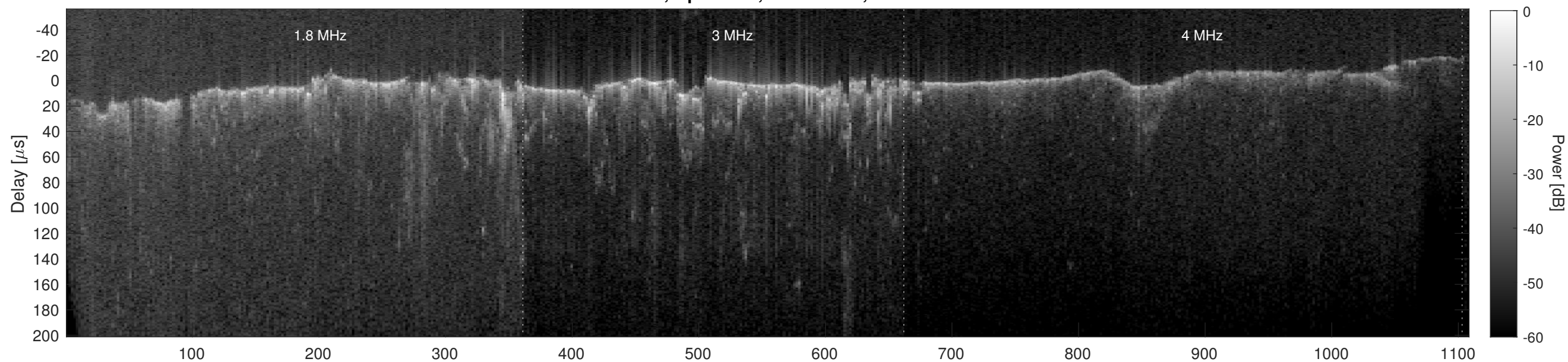
Orbit 6961, Cluttergram
