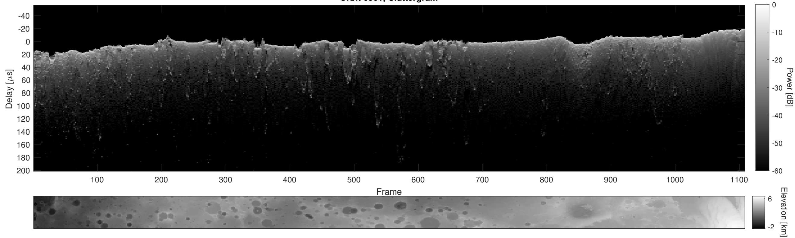
Orbit 6961, Cluttergram
