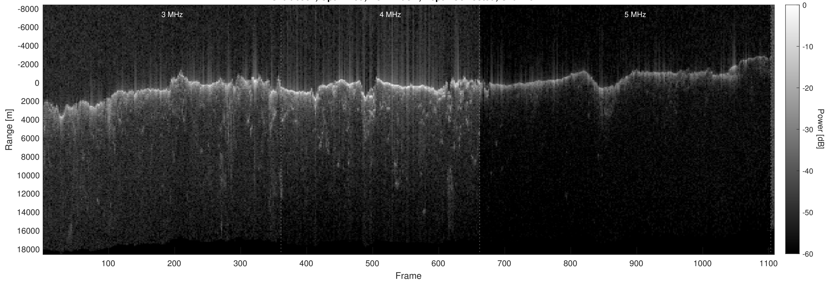
Orbit 6961, Optimized, No Window, Depth-Corrected, Channel 2
