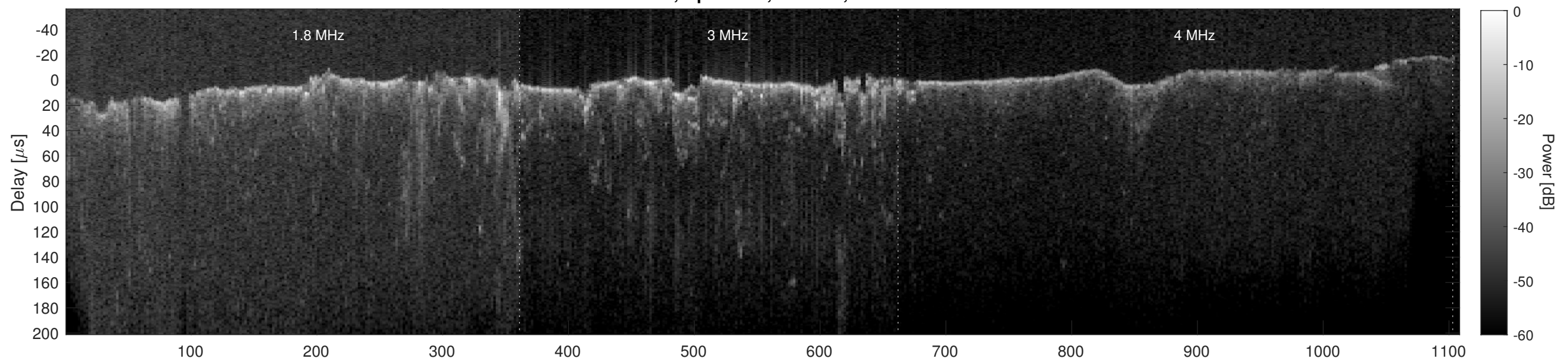
Orbit 6961, Cluttergram
