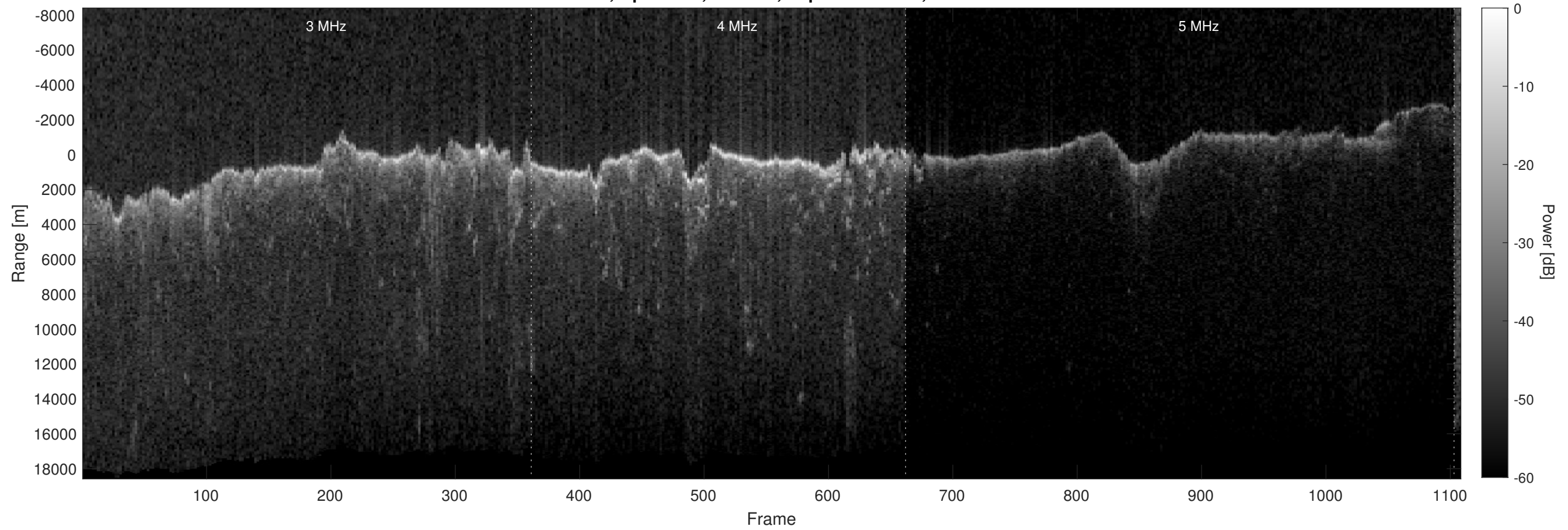
Orbit 6961, Optimized, Window, Depth-Corrected, Channel 2
