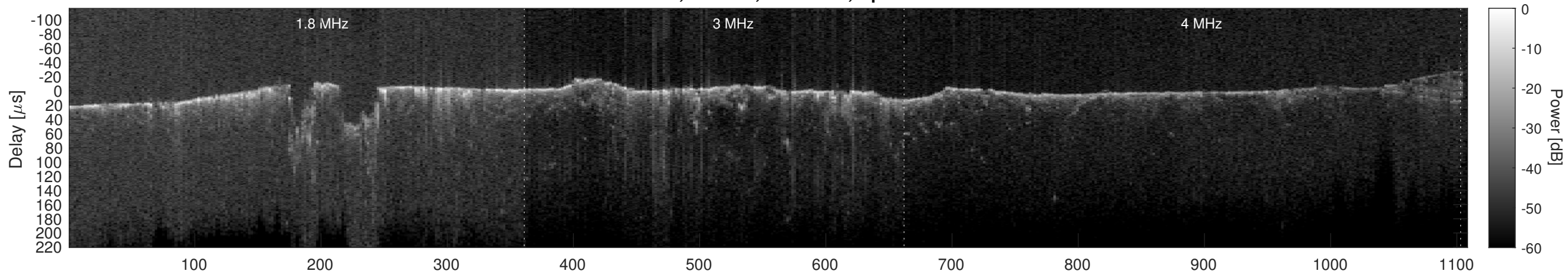
Orbit 6962, Cluttergram
