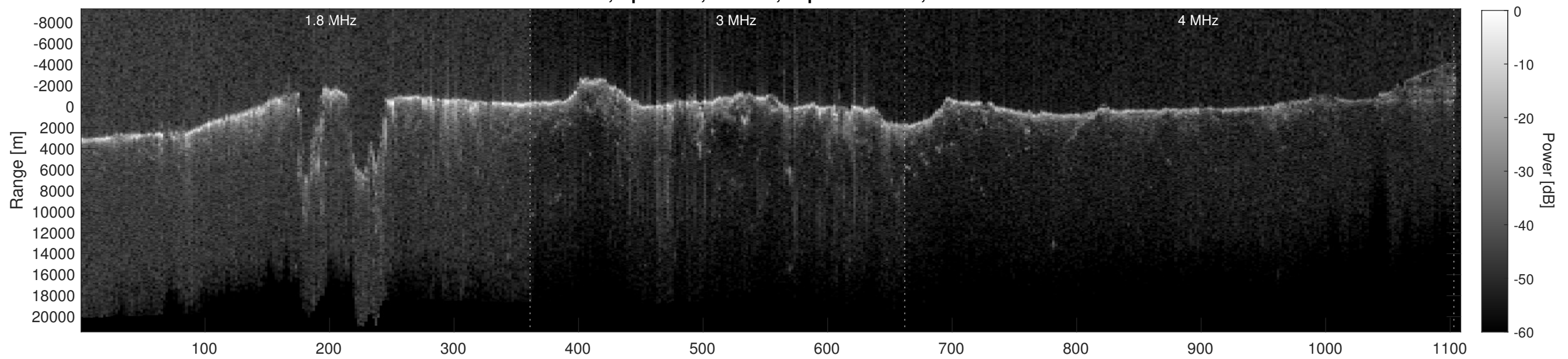
Orbit 6962, Depth-Corrected Cluttergram
