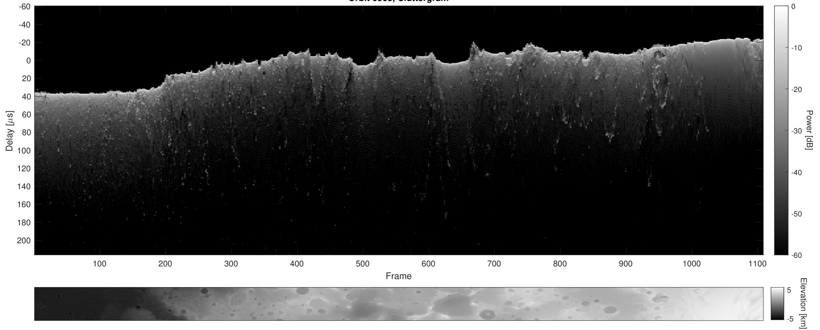
Orbit 6963, Cluttergram
