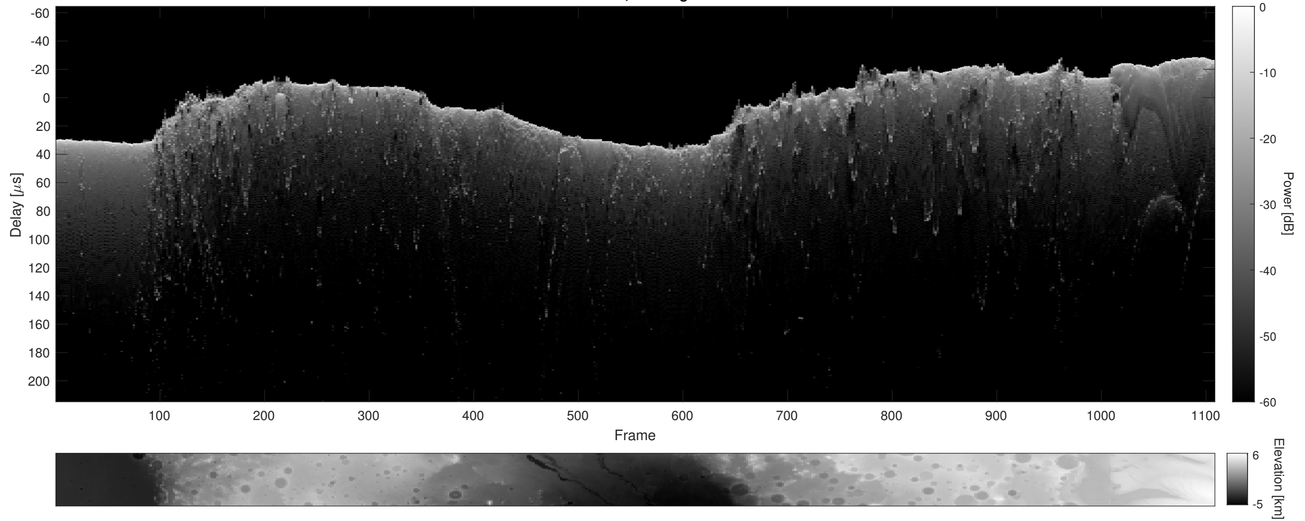
Orbit 6964, Cluttergram
