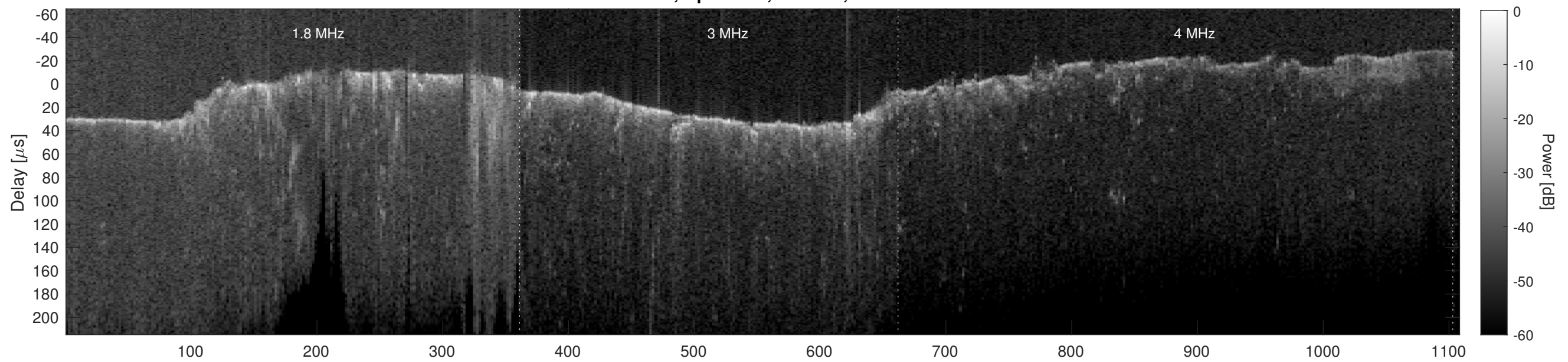
Orbit 6964, Cluttergram
