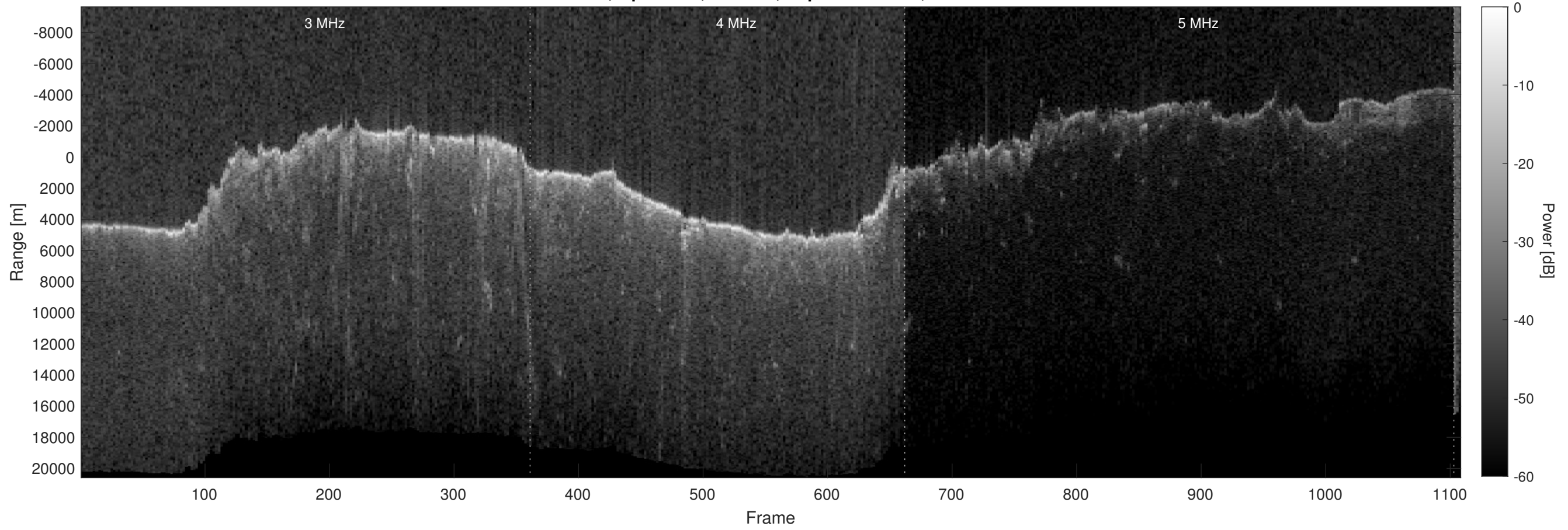
Orbit 6964, Optimized, Window, Depth-Corrected, Channel 2
