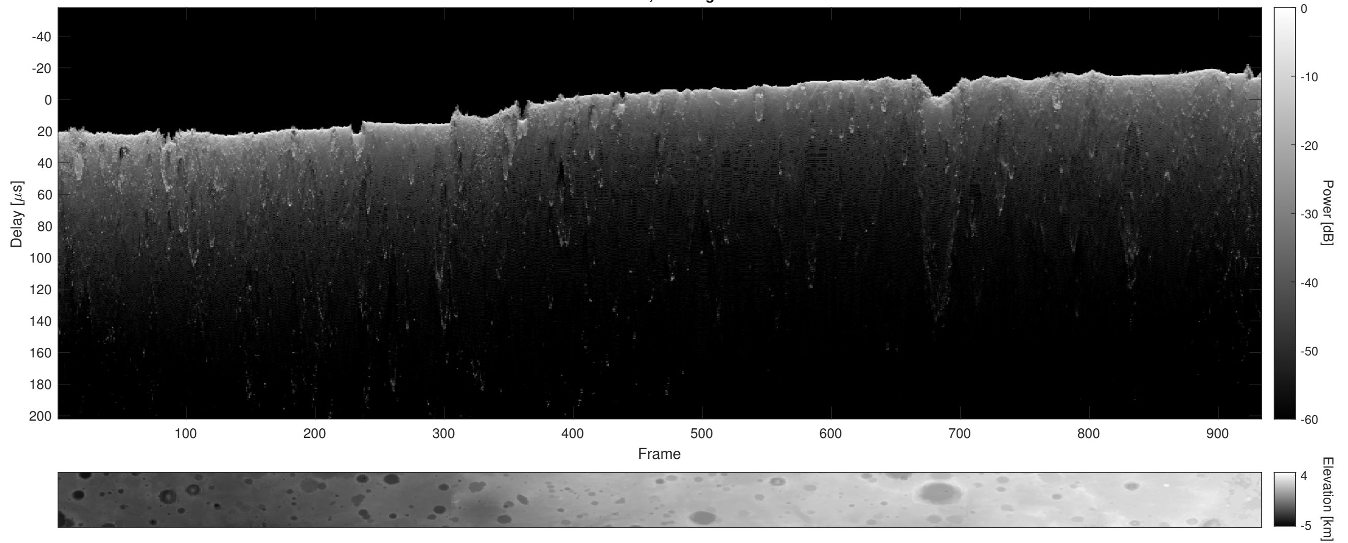
Orbit 6965, Cluttergram
