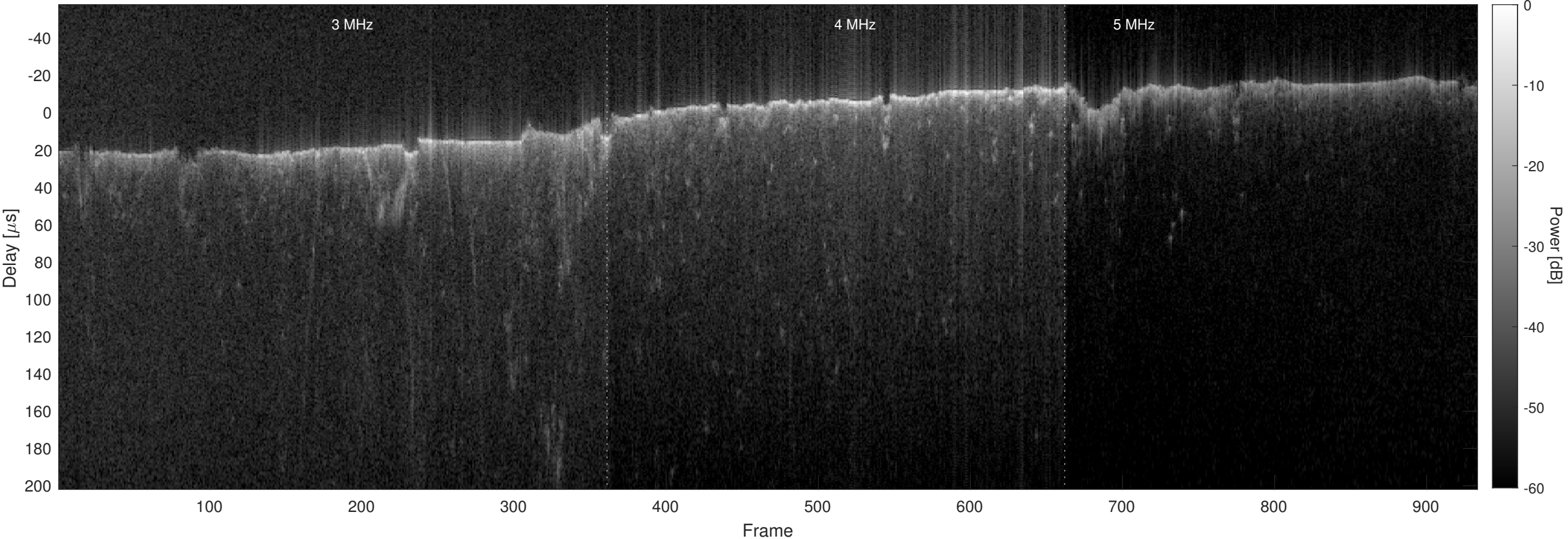
Orbit 6965, Optimized, No Window, Channel 2
