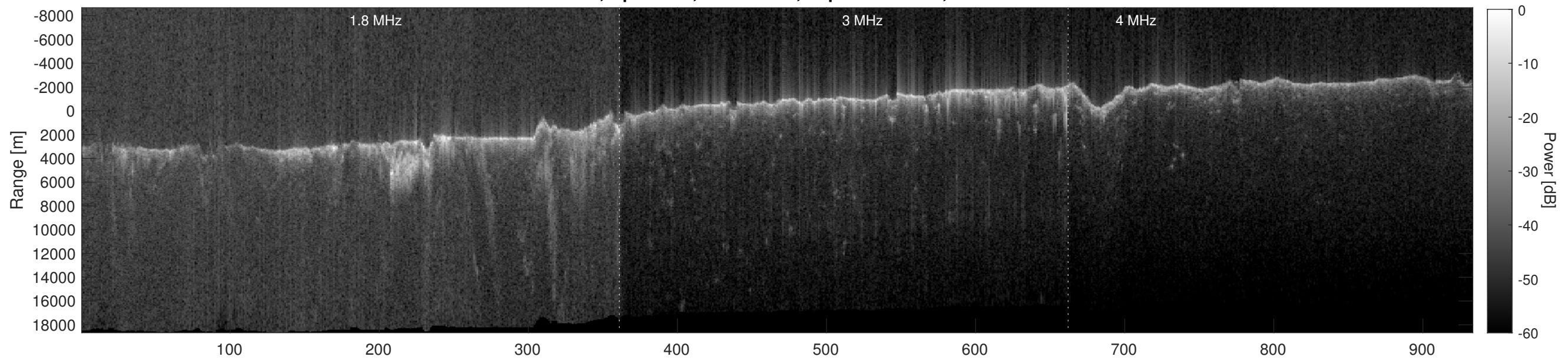
Orbit 6965, Depth-Corrected Cluttergram
