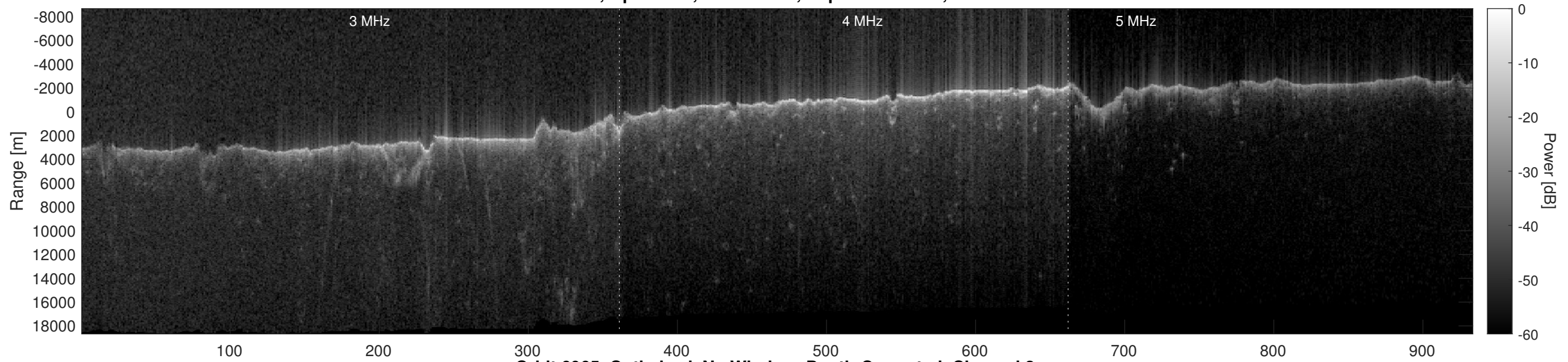
Orbit 6965, Optimized, No Window, Depth-Corrected, Channel 2
