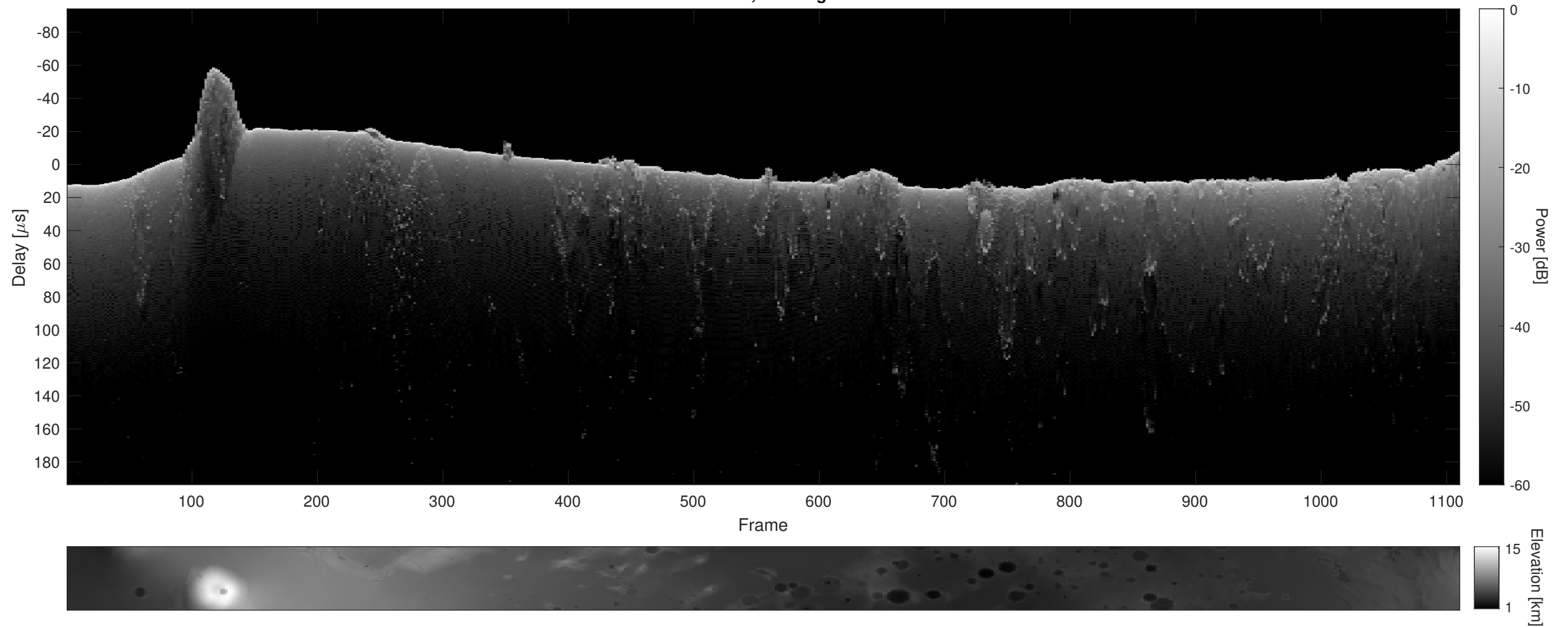
Orbit 6966, Cluttergram
