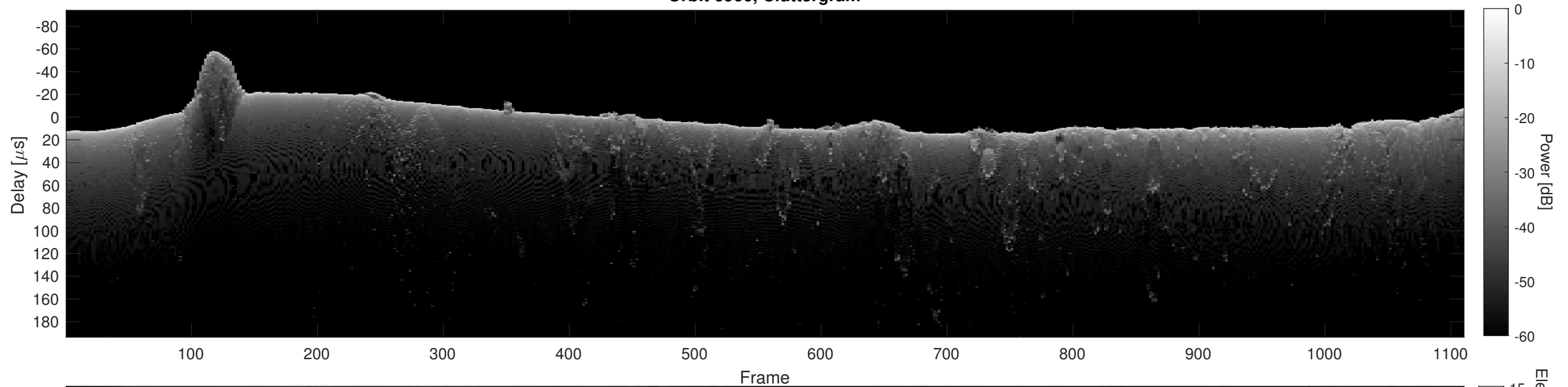
Orbit 6966, Cluttergram
