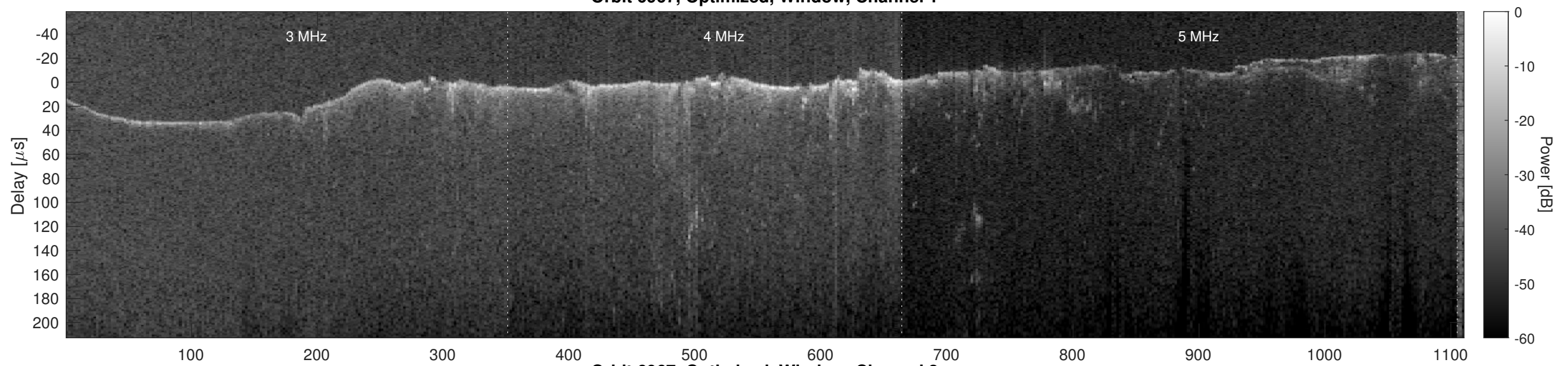
Orbit 6967, Optimized, Window, Channel 2
