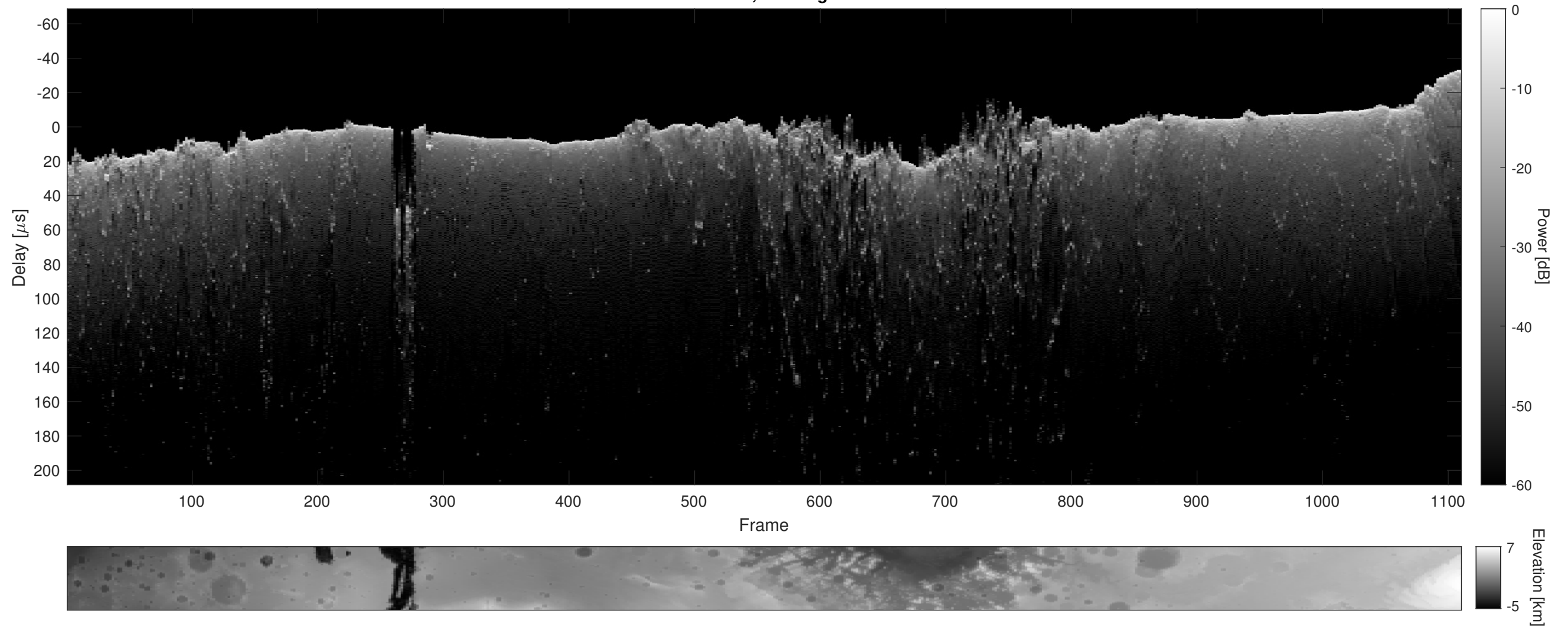
Orbit 6969, Cluttergram
