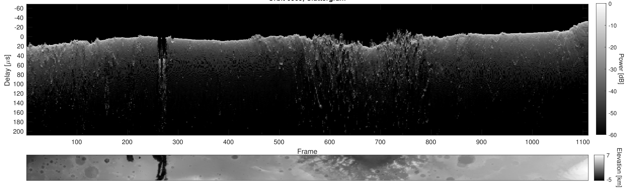
Orbit 6969, Cluttergram
