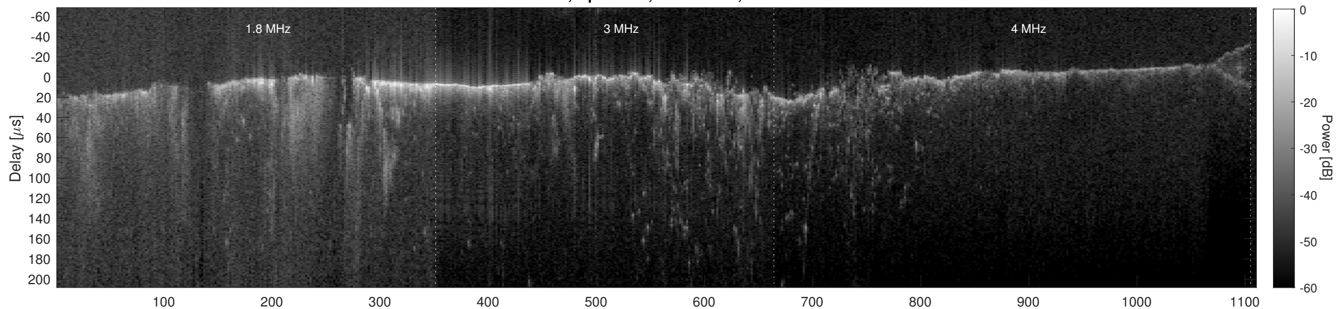
Orbit 6969, Cluttergram
