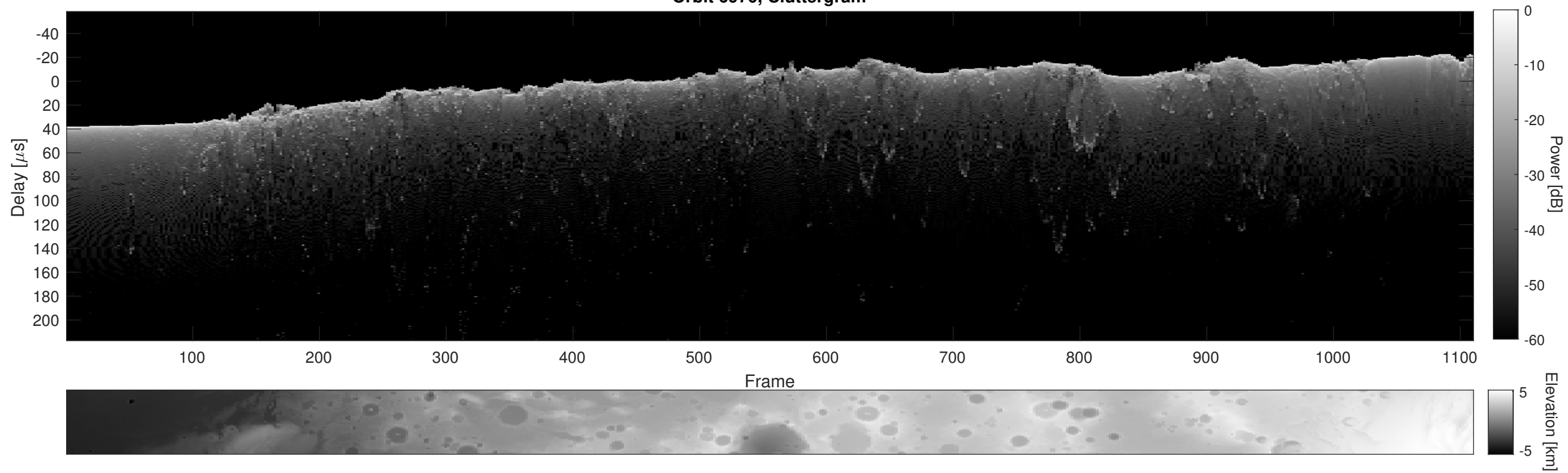
Orbit 6970, Cluttergram
