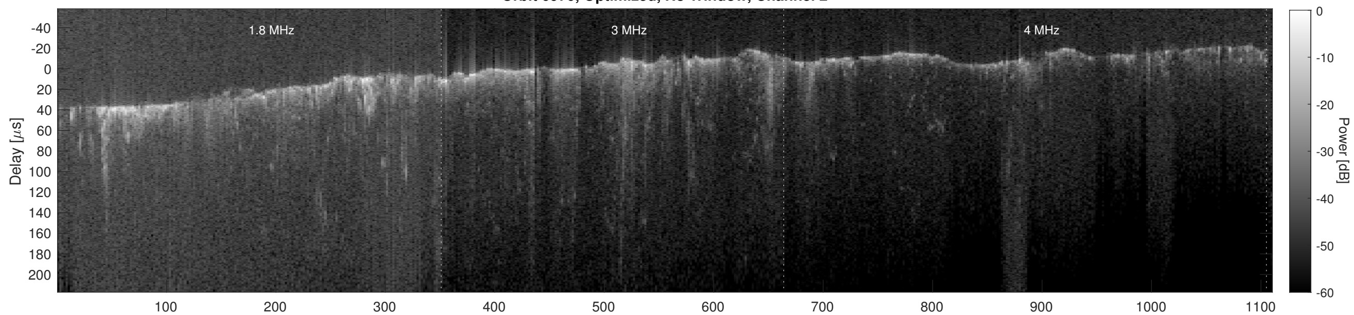
Orbit 6970, Cluttergram
