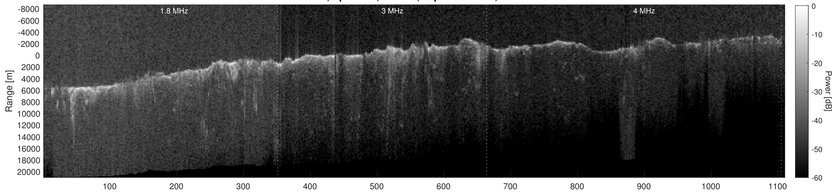
Orbit 6970, Depth-Corrected Cluttergram
