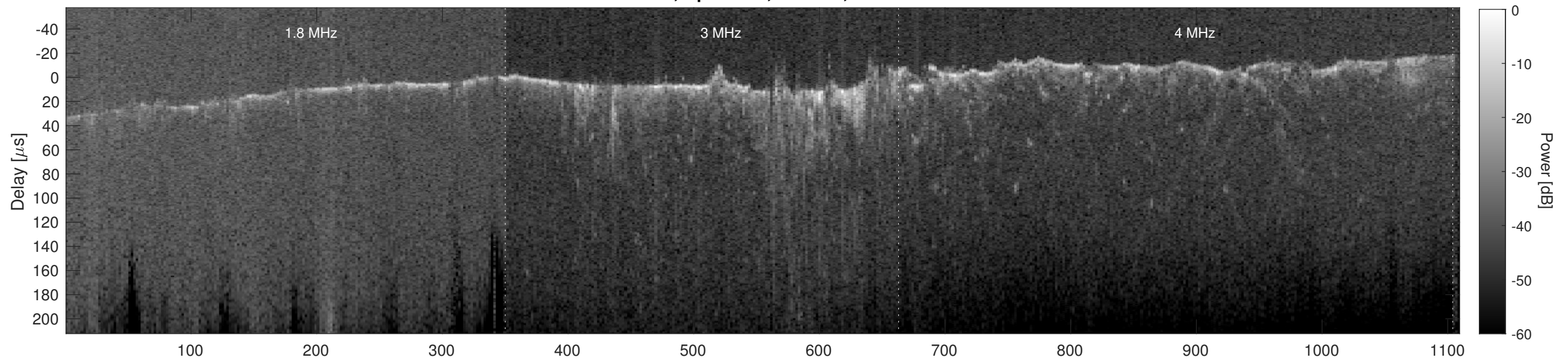
Orbit 6971, Cluttergram
