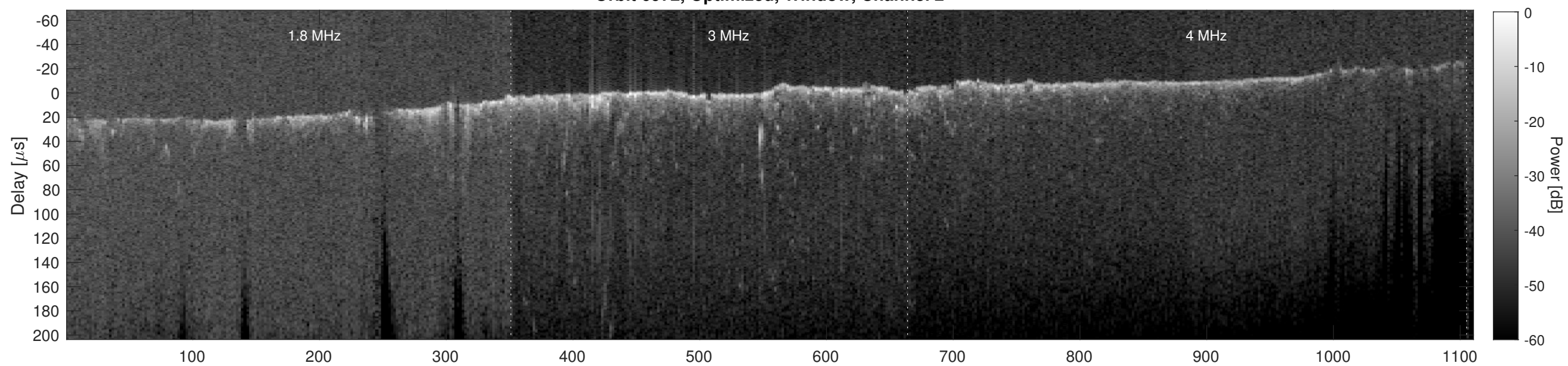
Orbit 6972, Cluttergram
