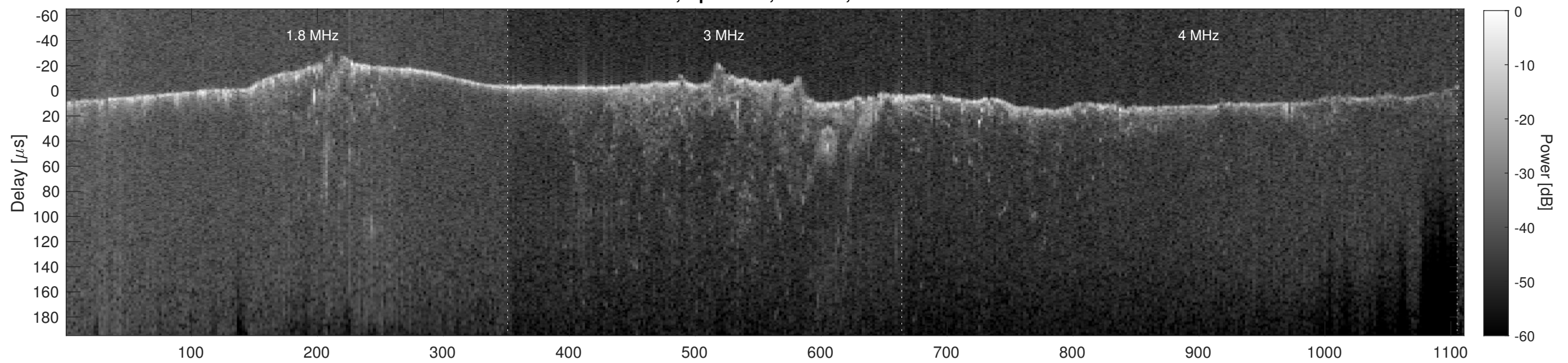
Orbit 6973, Cluttergram
