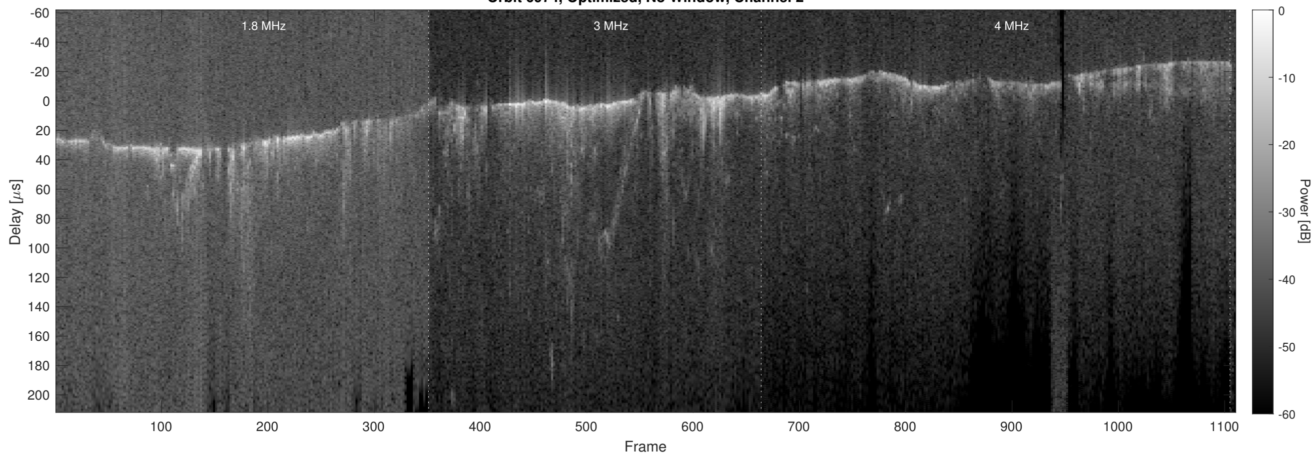
Orbit 6974, Optimized, No Window, Channel 2
