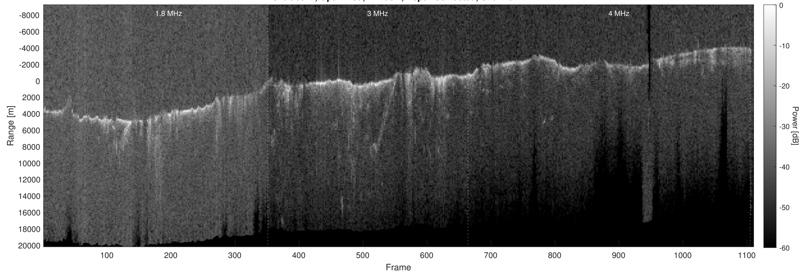
Orbit 6974, Optimized, Window, Depth-Corrected, Channel 2
