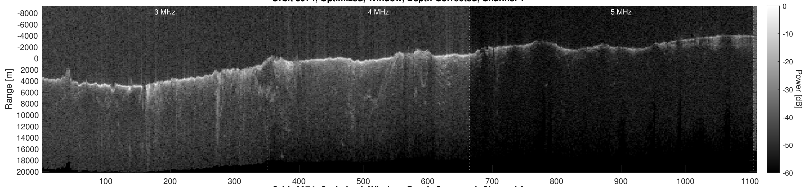
Orbit 6974, Optimized, Window, Depth-Corrected, Channel 2
