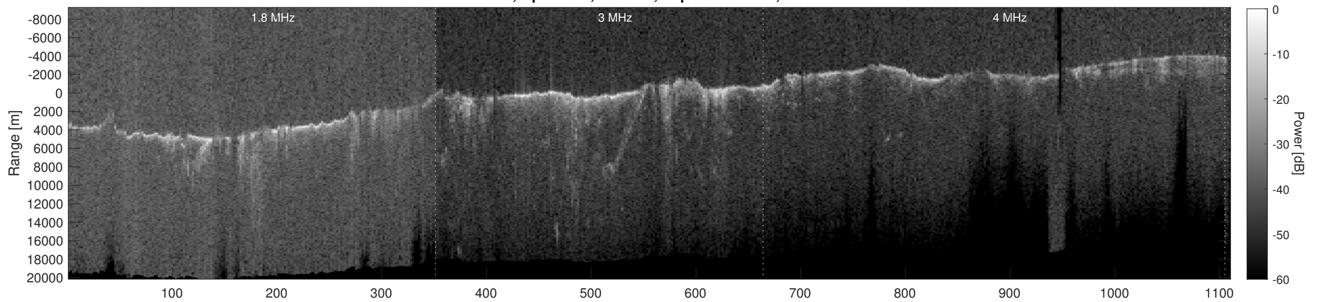
Orbit 6974, Depth-Corrected Cluttergram
