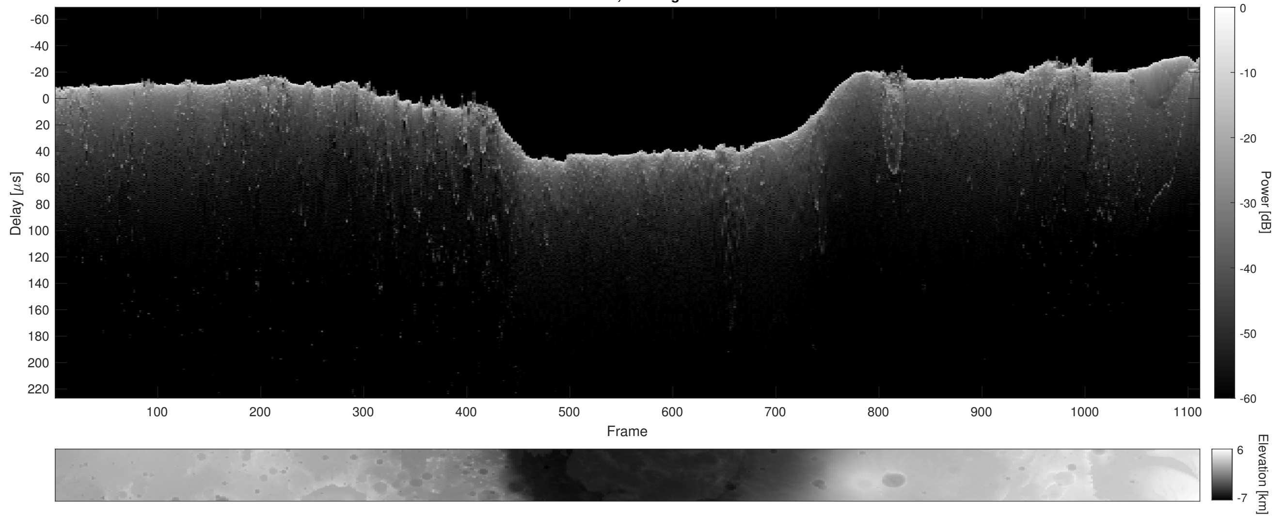
Orbit 6975, Cluttergram
