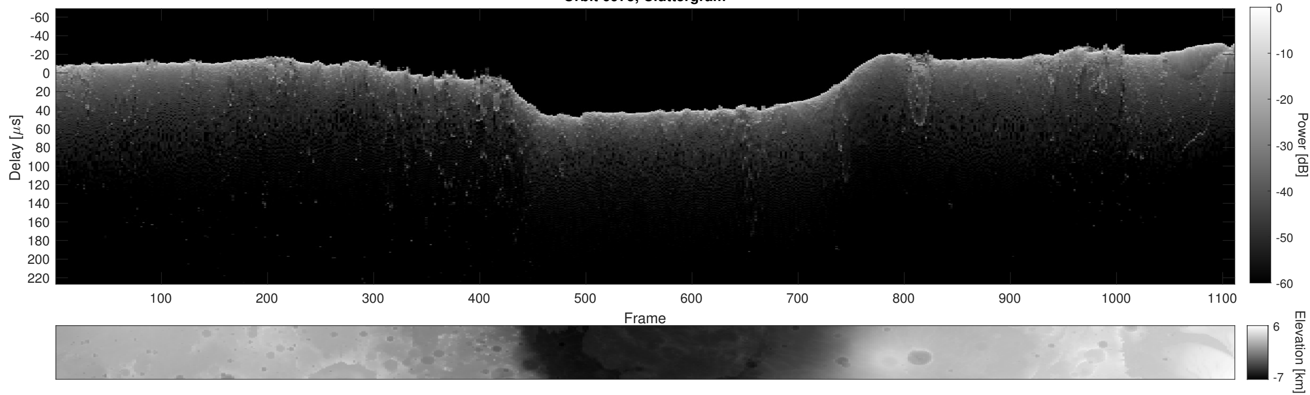
Orbit 6975, Cluttergram
