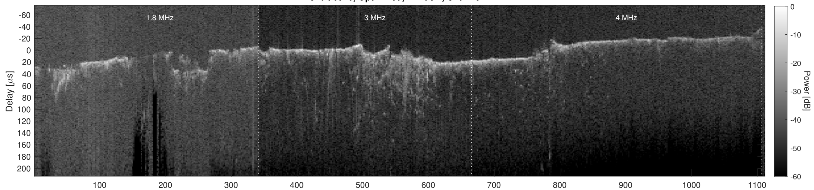
Orbit 6976, Cluttergram
