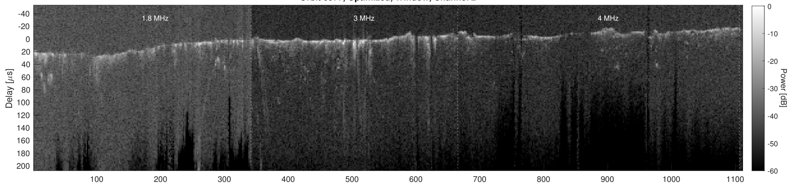
Orbit 6977, Cluttergram
