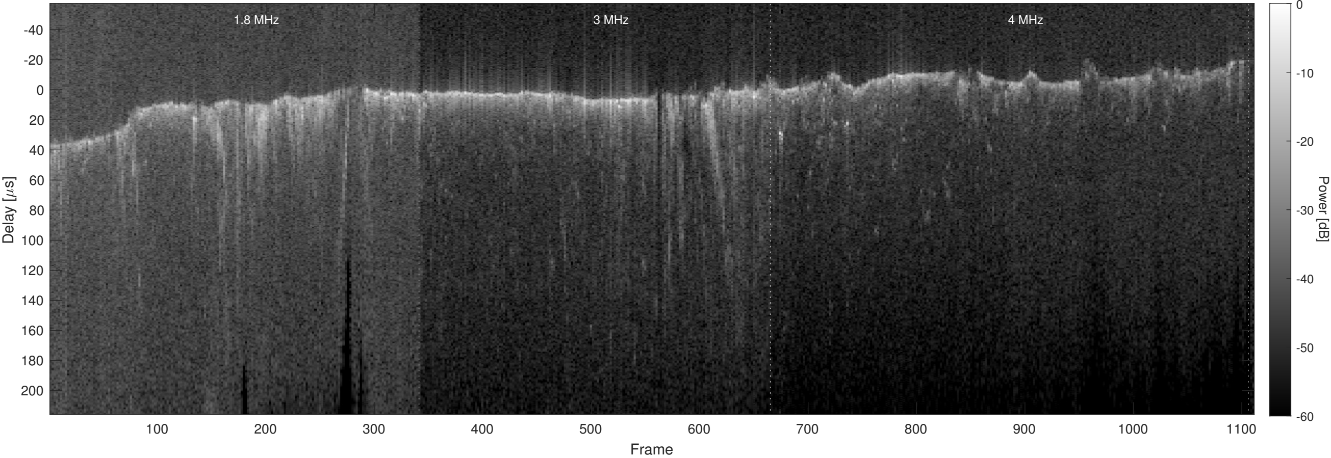
Orbit 6978, Optimized, No Window, Channel 2
