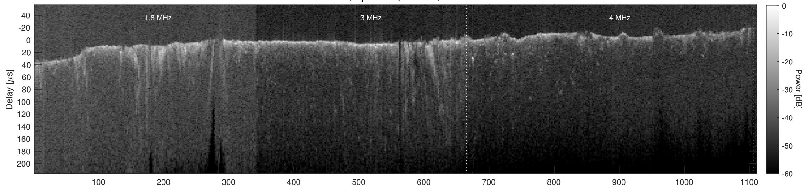
Orbit 6978, Cluttergram
