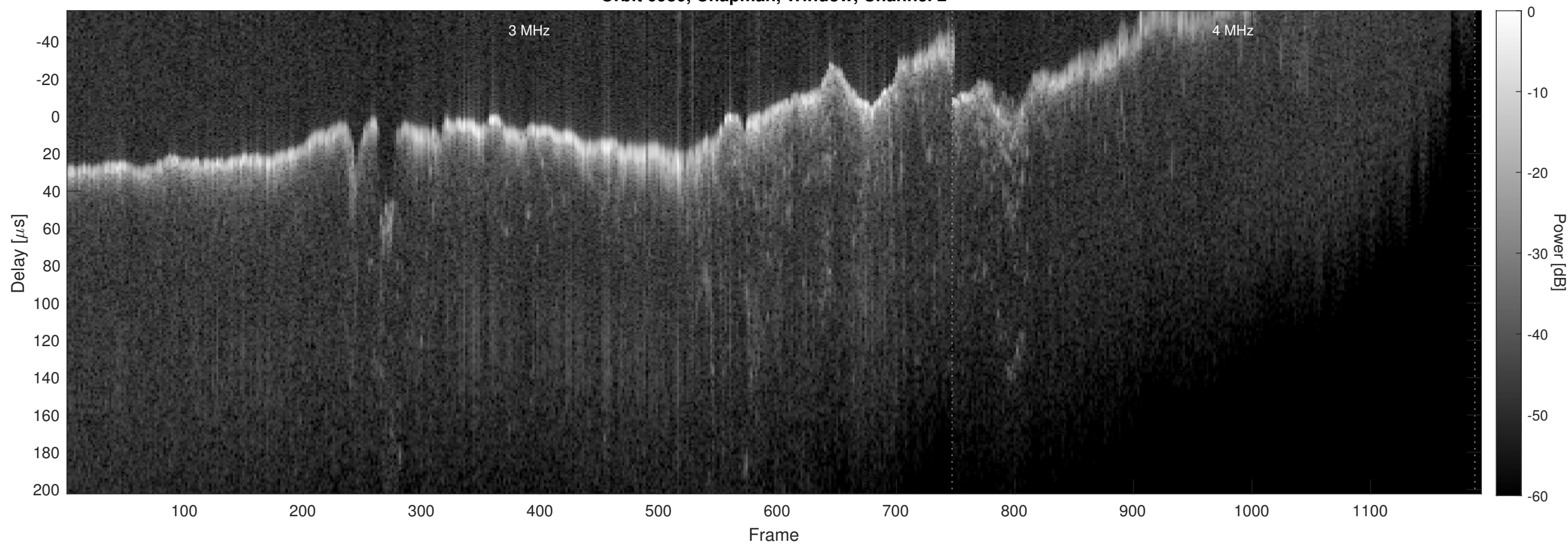
Orbit 6980, Chapman, Window, Channel 2
