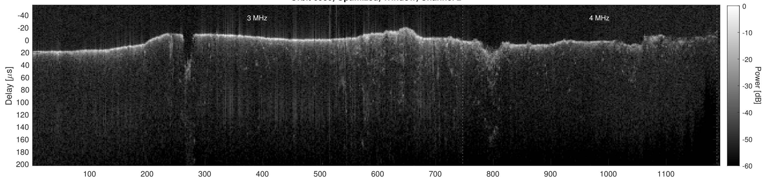
Orbit 6980, Cluttergram
