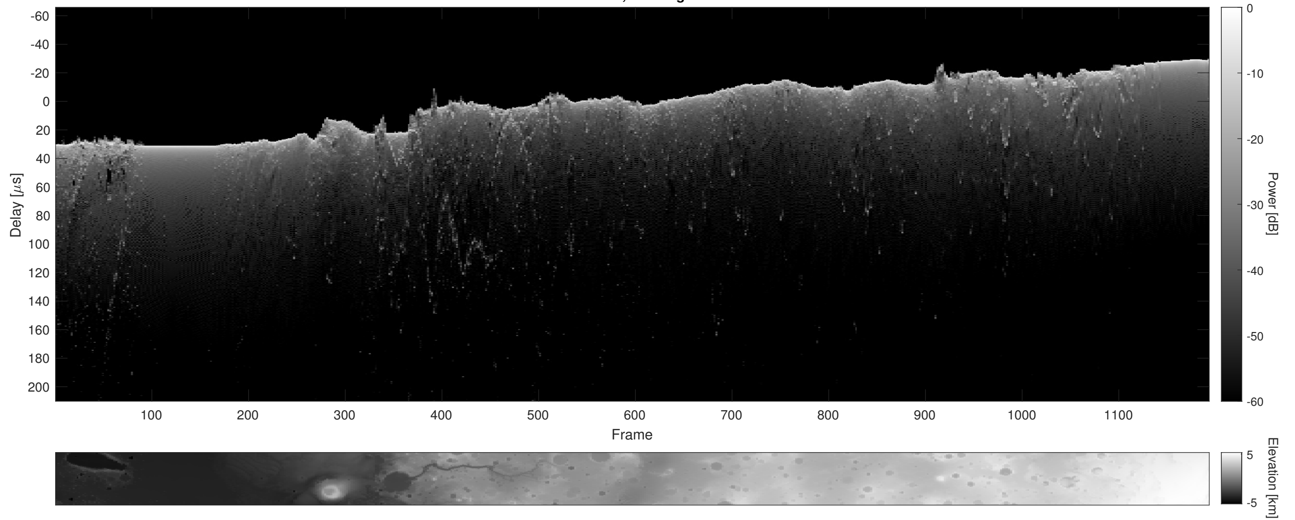
Orbit 6981, Cluttergram
