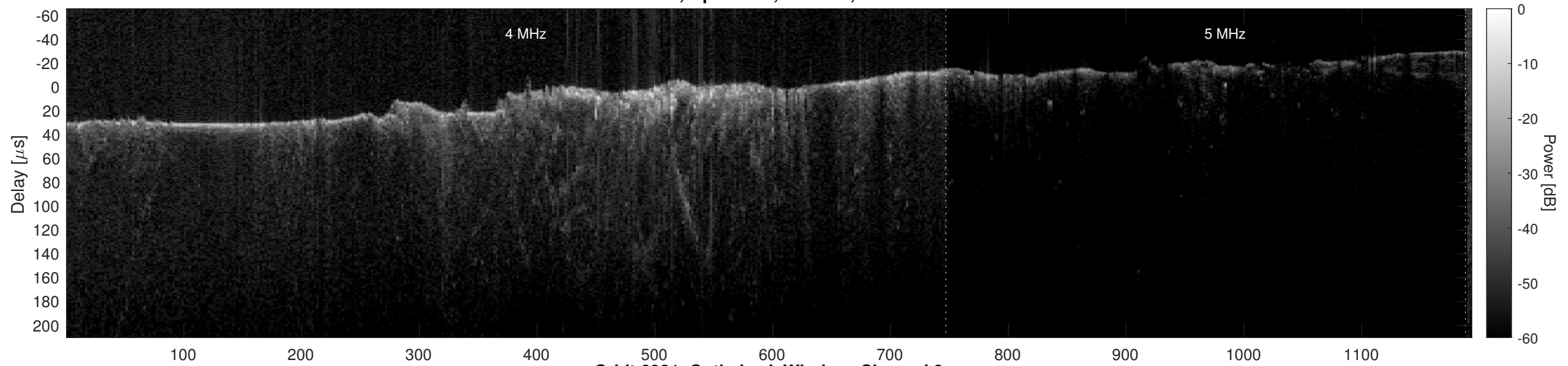
Orbit 6981, Optimized, Window, Channel 2
