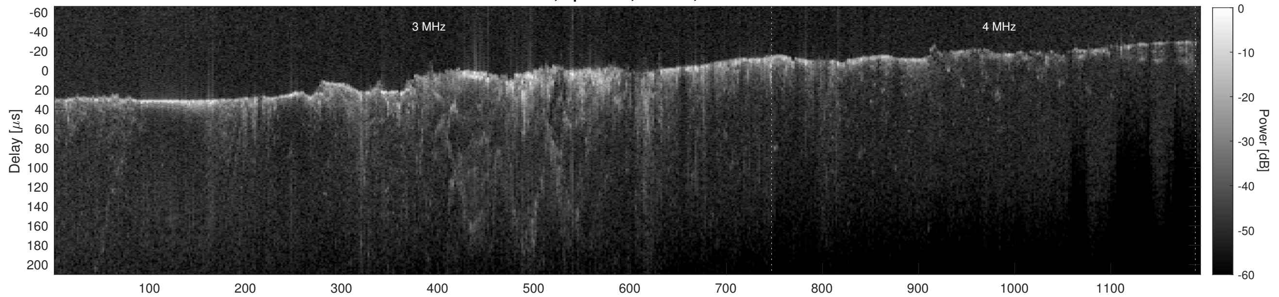
Orbit 6981, Cluttergram
