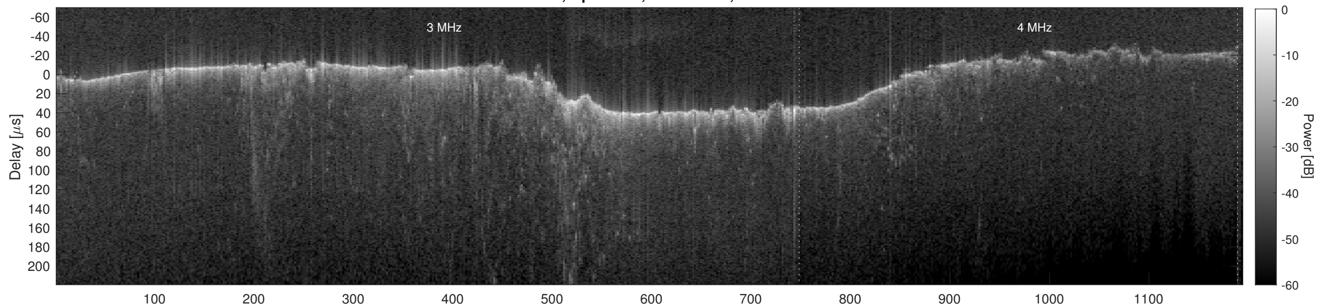
Orbit 6982, Cluttergram
