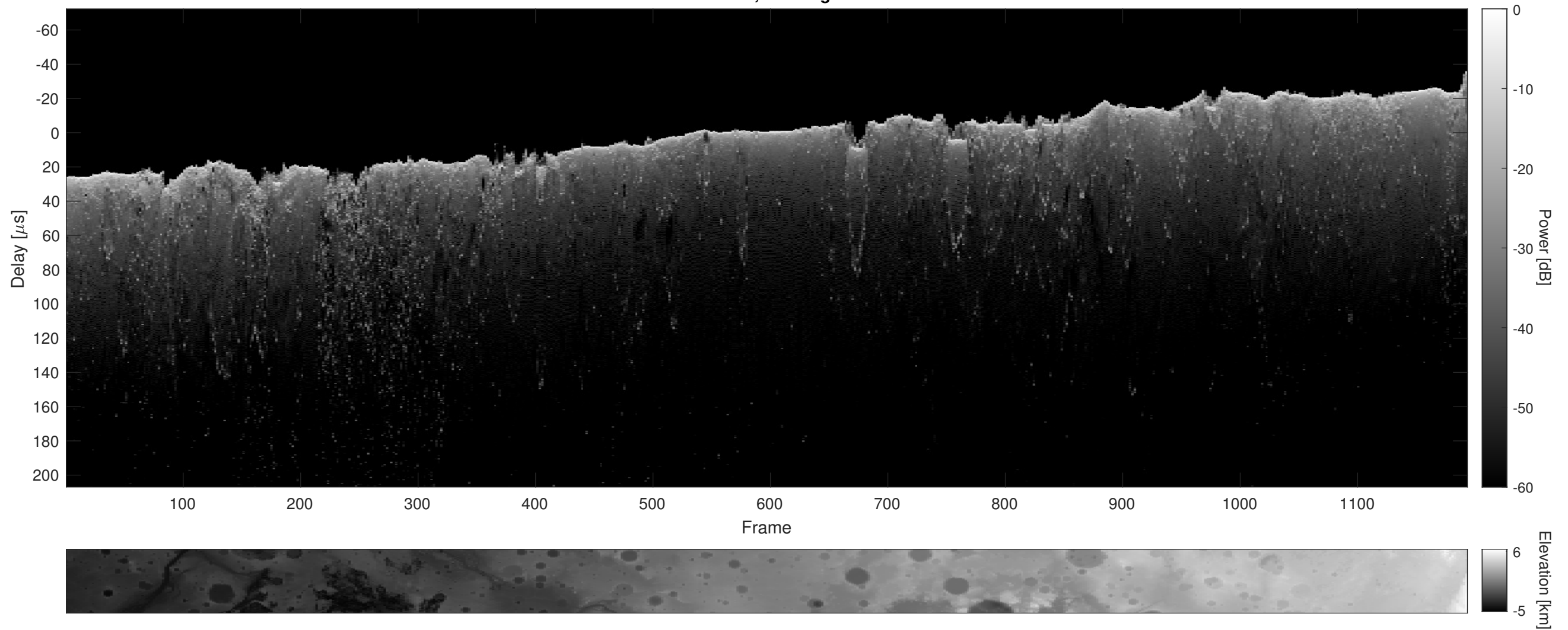
Orbit 6983, Cluttergram
