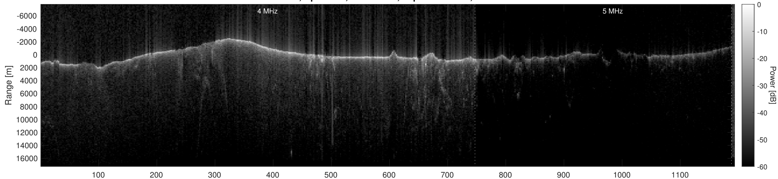
Orbit 6984, Optimized, No Window, Depth-Corrected, Channel 2
