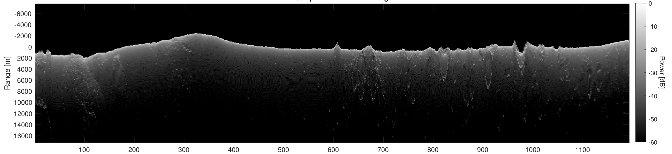
Orbit 6984, Depth-Corrected Cluttergram
