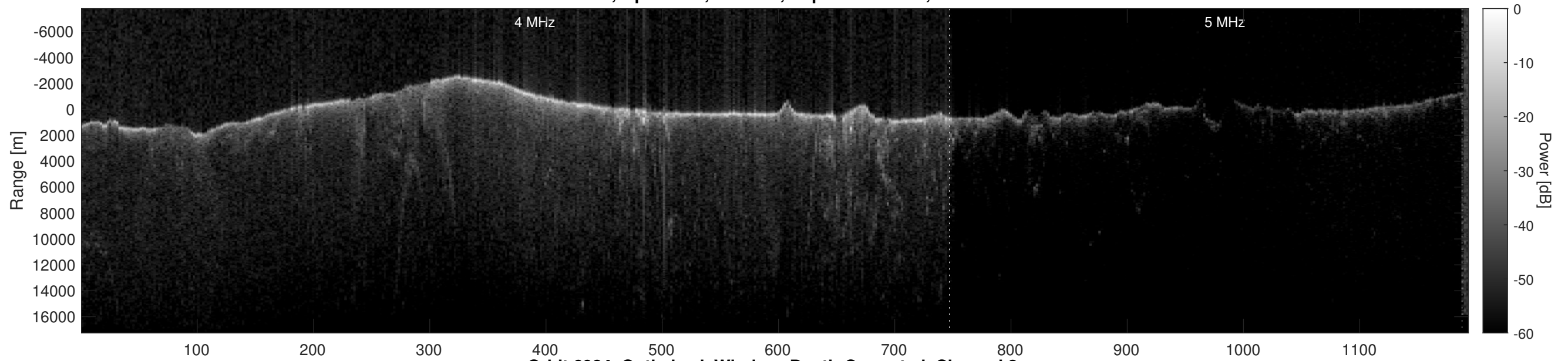
Orbit 6984, Optimized, Window, Depth-Corrected, Channel 2
