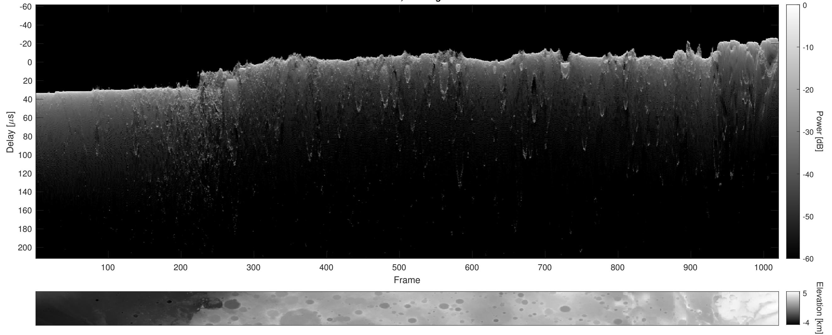
Orbit 6985, Cluttergram
