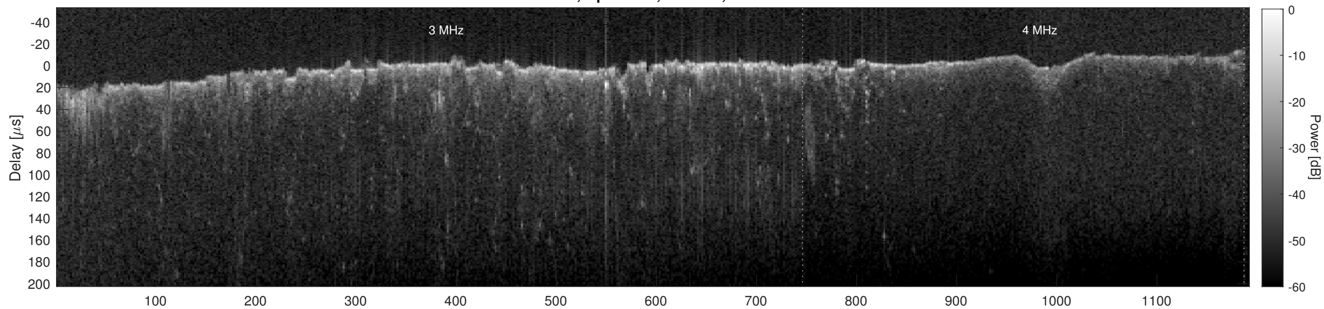
Orbit 6986, Cluttergram
