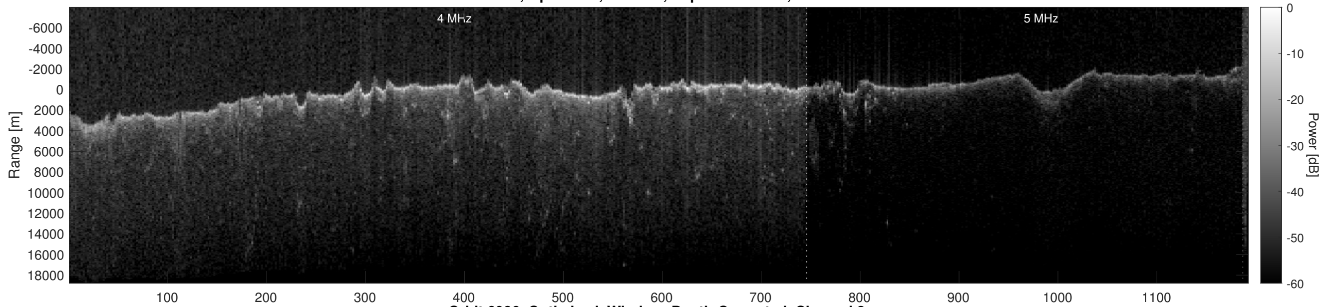
Orbit 6986, Optimized, Window, Depth-Corrected, Channel 2
