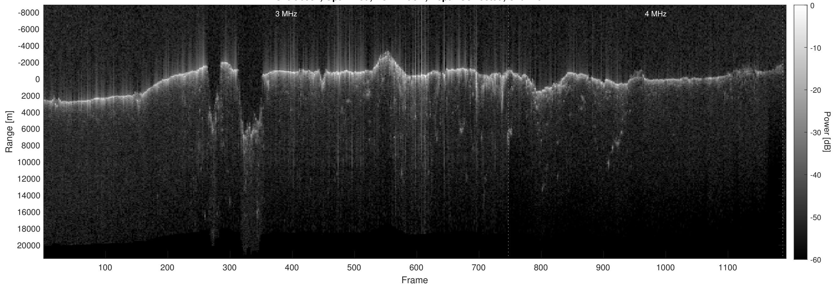
Orbit 6987, Optimized, No Window, Depth-Corrected, Channel 2
