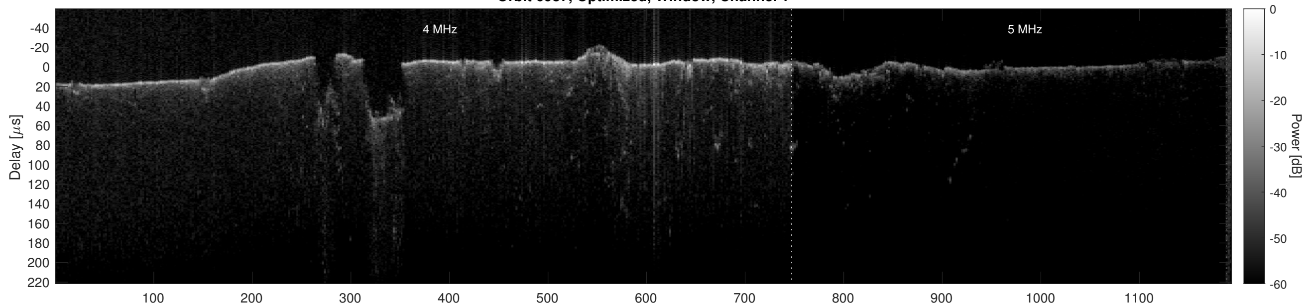
Orbit 6987, Optimized, Window, Channel 2
