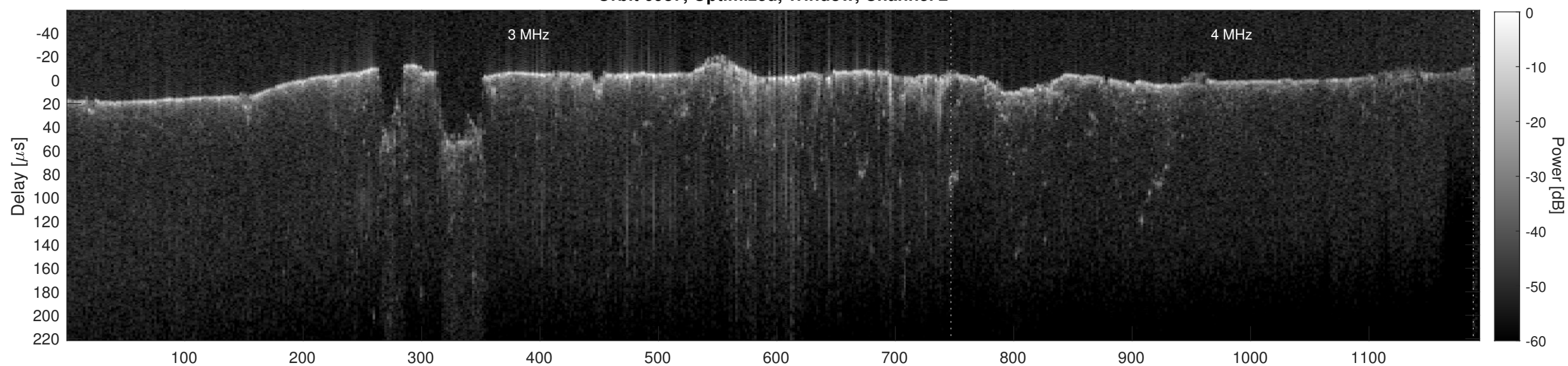
Orbit 6987, Cluttergram
