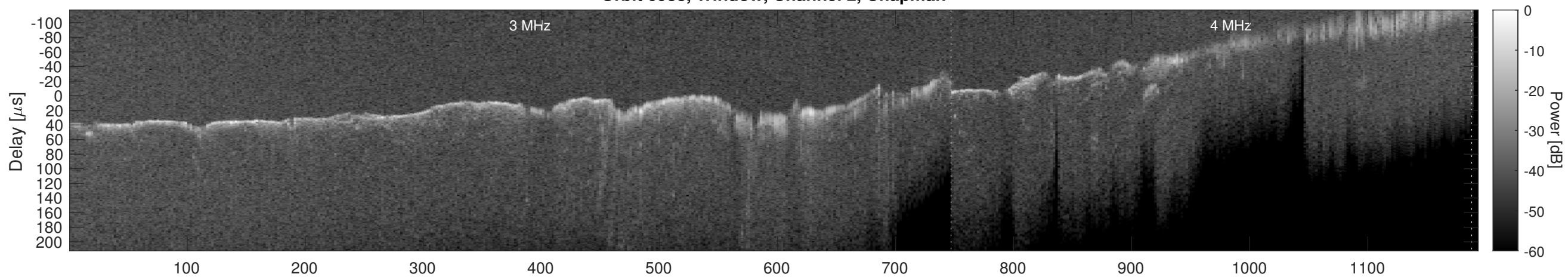
Orbit 6988, Window, Channel 2, Optimized
