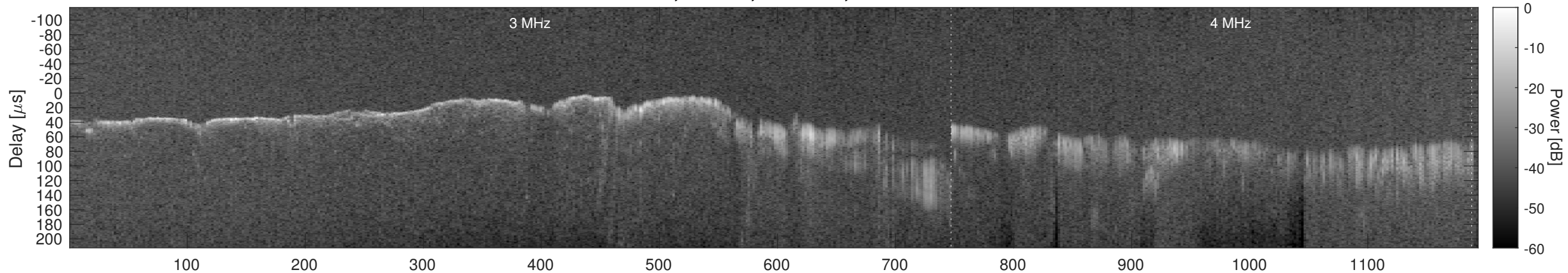
Orbit 6988, Window, Channel 2, Chapman
